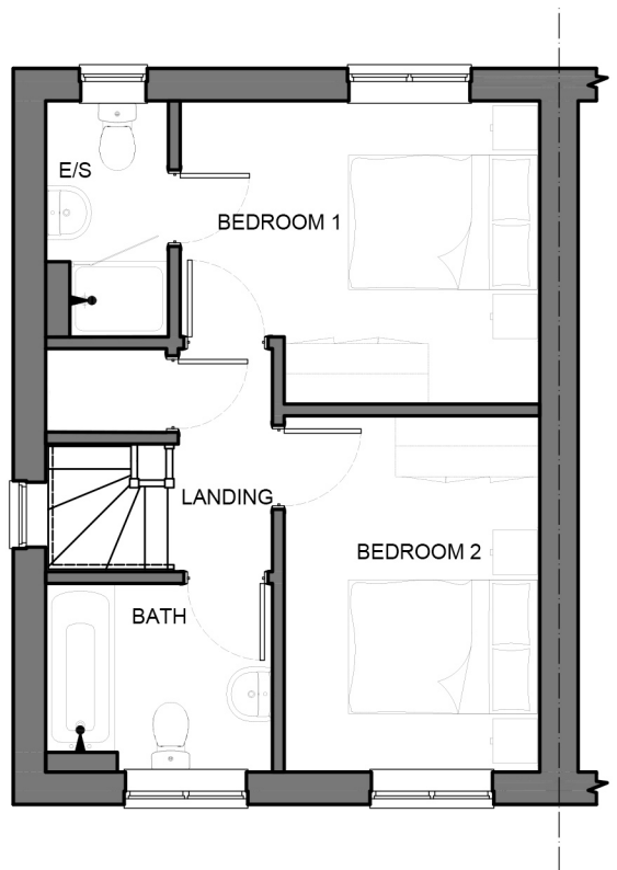
FIRST FLOOR PLAN (OPTIONAL EN-SUITE)
